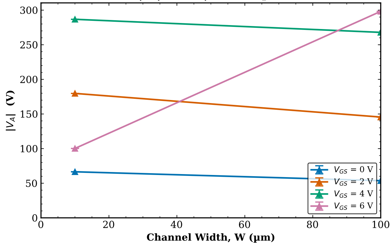
TFT3 Transistor 2 |V_A| vs W | L = 80\text{ }\mu\text{m}
